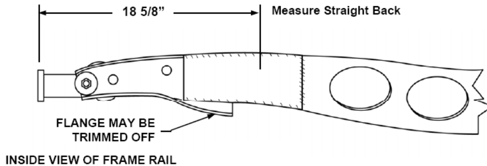
Figure 1- Boxing Frame & Axle Centerline
