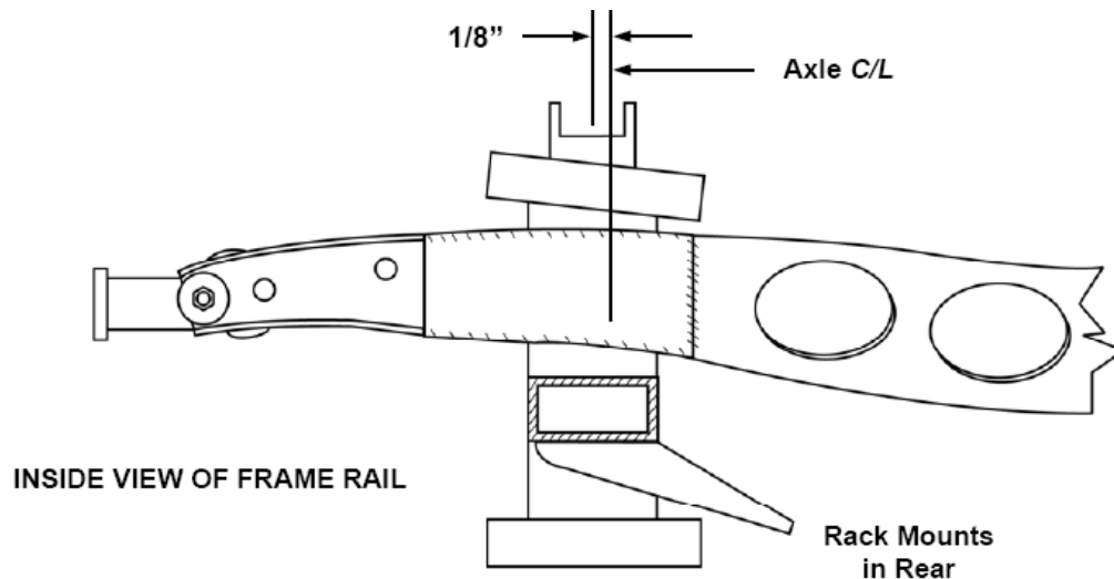
Figure 2- Crossmember Fitment
