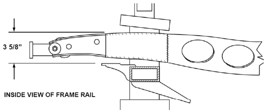
Figure 3- Radiator Support Bracket Install
